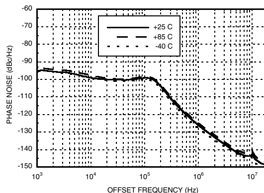
Phase Noise @ 2 GHz, Integer Mode
