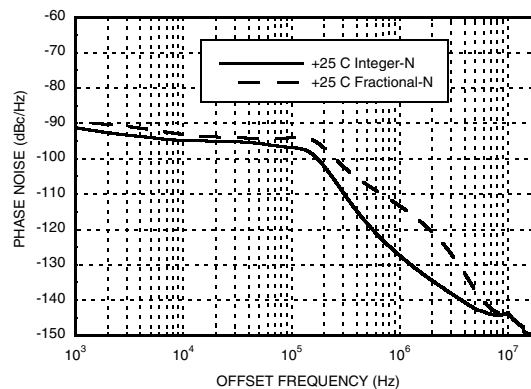
Phase Noise @ 4 GHz Integer vs. Fractional Mode
